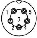
5 PIN
