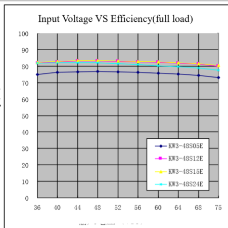
Input Voltage(Vdc) Photo10
