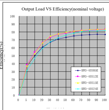
Output Load(%) Photo 12
