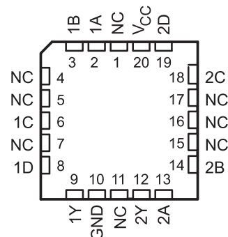
SN54ALS21A, SN54AS21 . . . FK PACKAGE (TOP VIEW)
