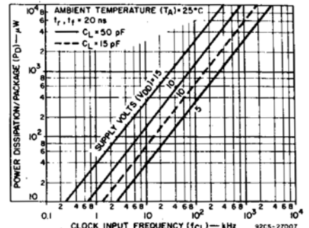
Fig. 9 - Typical dynamic power dissipation vs. frequency.
