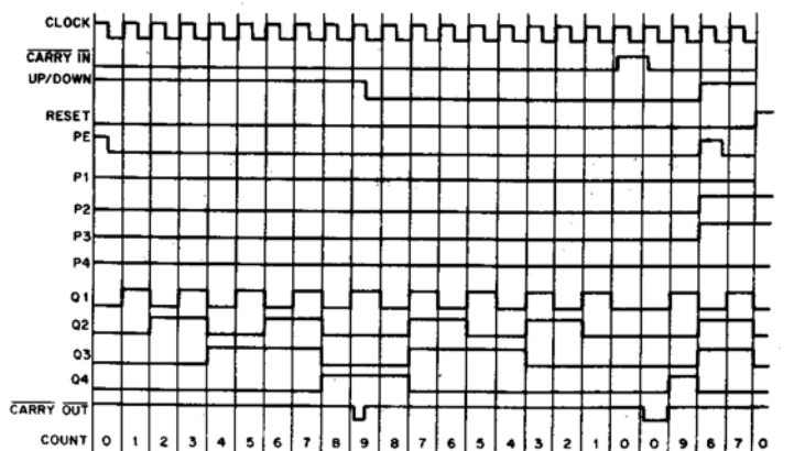
Fig. 15 — Timing Diagram for CD4510B.
