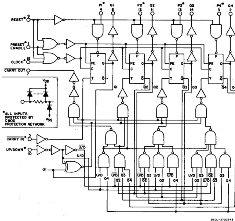
Fig.3 - Logic Diagram for CD4510B.
